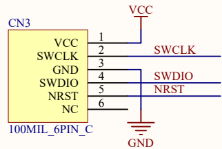
SWD Interface
